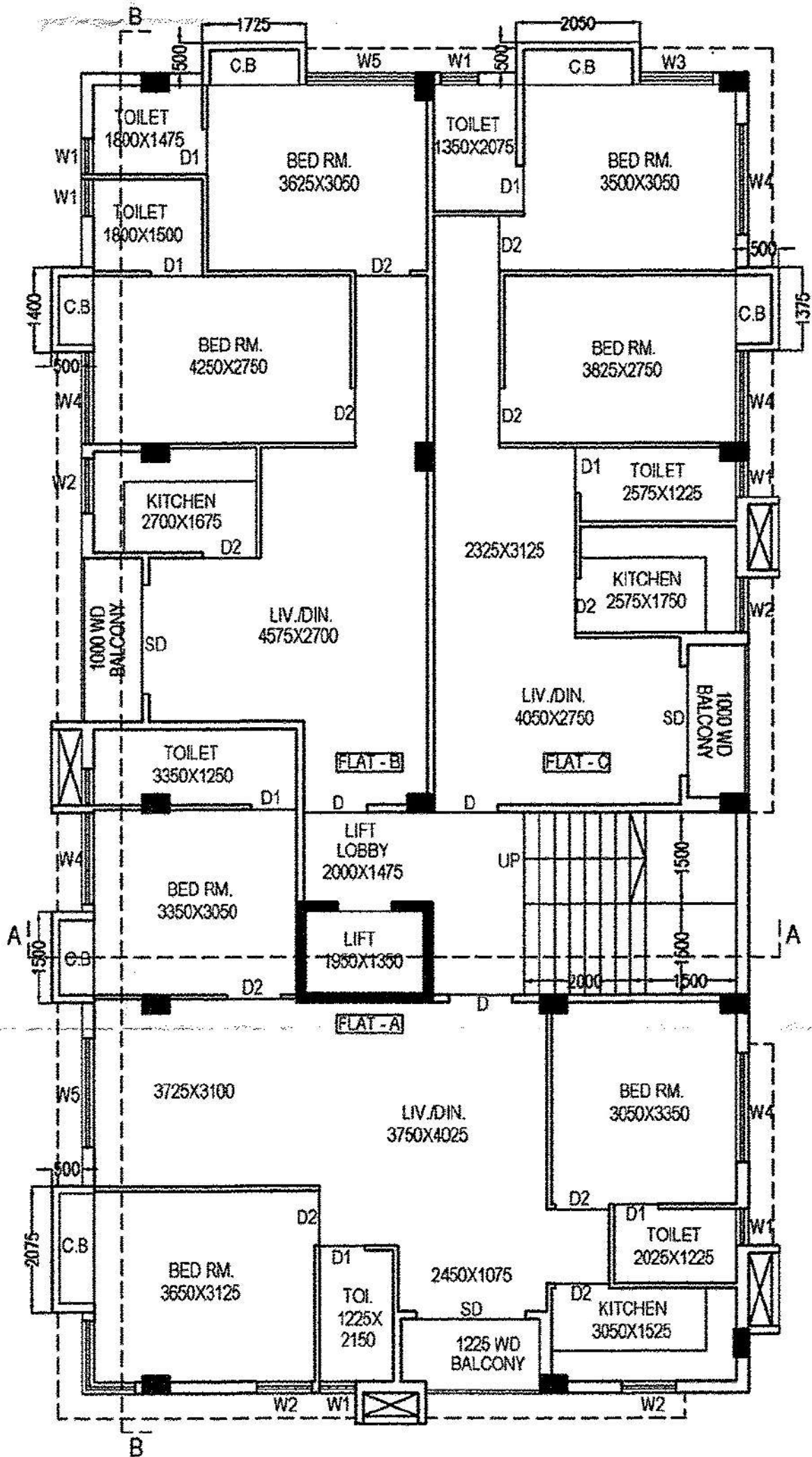
2ND , 3RD FLOOR PLAN
